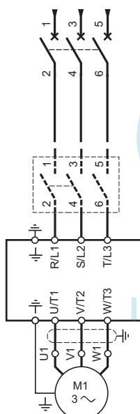
Motor starter with three-phase power supply
