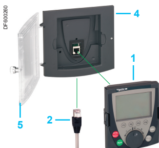
Using the remote graphic display terminal on enclosure door: 1 + 2 + 4 (+ 5, if IP 65)
