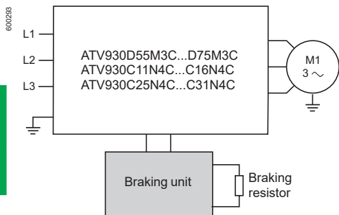
Altivar Process drive with braking unit
