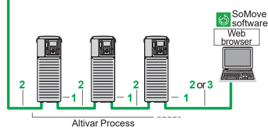
Example of connection on an EtherNet/IP network
