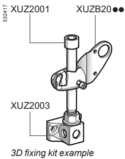
3D fixing kit example
