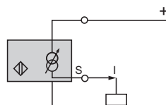
3-wire connection
