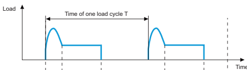
Motor service duty S4
