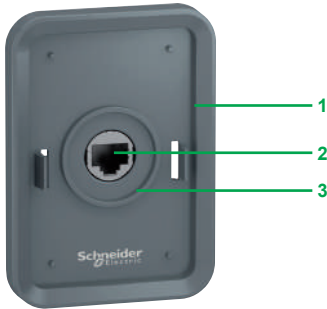
Remote-mounting kit VW3A1114 (front view)
