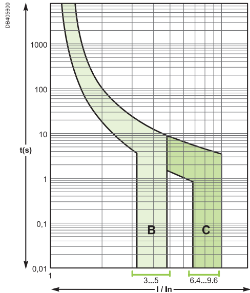
Time current tripping curves
