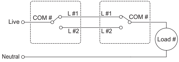
2-way Switch – 4G
