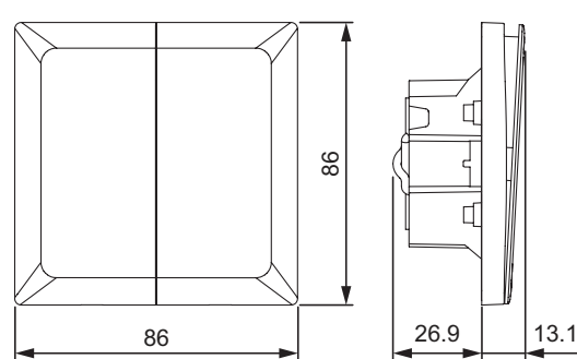
2G Intermediate Switch
