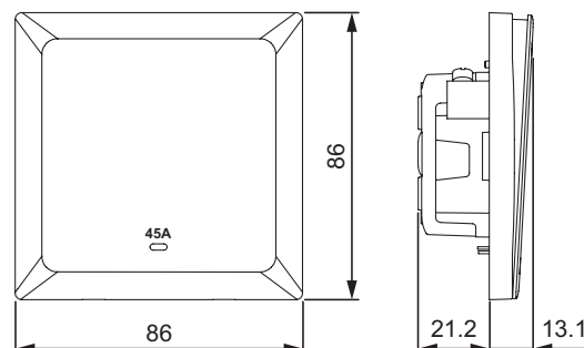
1G Double Pole Switch with LED Indicator – 45 A
