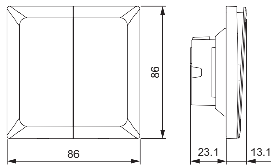
2G Switch, Momentary Switch
