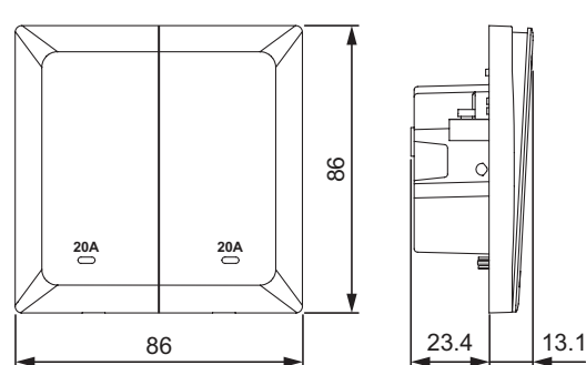
2G Switch with LED Indicator – 20 A
