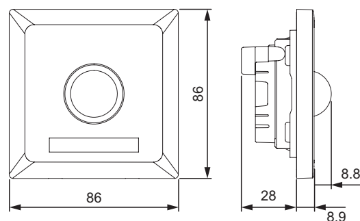
Night Foot Lamp with PIR Sensor
